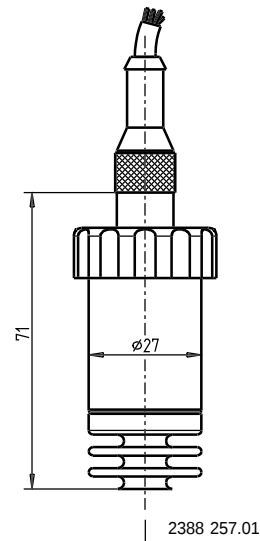
locking plug, 4-pin M 12 x 1, IP 67
